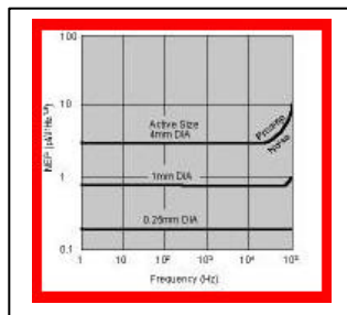
Noise Equivalent Power (NEP) vs Frequency
